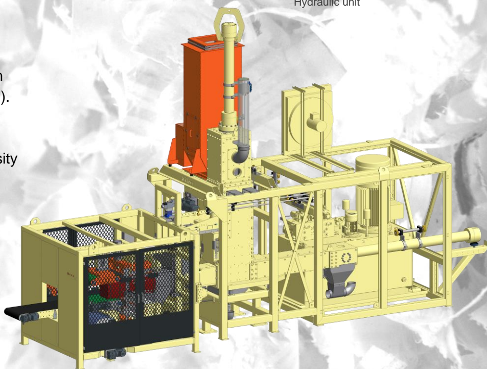
Hydraulic unit
